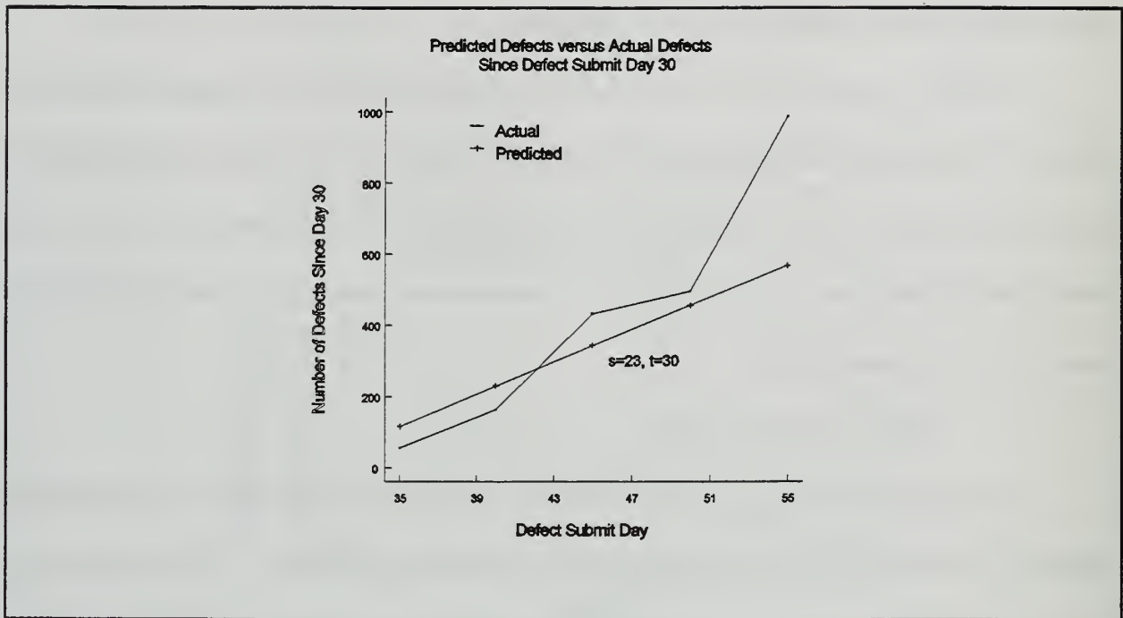
Figure 14. Predicted Defects vs Actual Defects
