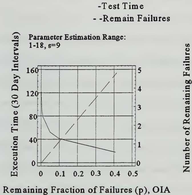
Figure 4: Test Time for Given Remaining Failures
